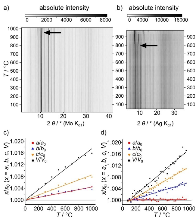
Figure 6. Thermal stability measurements and thermal expansion. a) Variable temperature powder X-ray diffractograms of \text{LiP}_4\text{N}_7 measured from 40–1000 °C with Mo K_{\alpha 1} radiation. An arrow marks beginning decomposition. b) Variable temperature powder X-ray diffractogram of \text{Li}_{3-x}\text{P}_6\text{N}_{11-x}(\text{NH})_x measured from 60–900 °C with Ag K_{\alpha 1} radiation. An arrow marks beginning decomposition.
